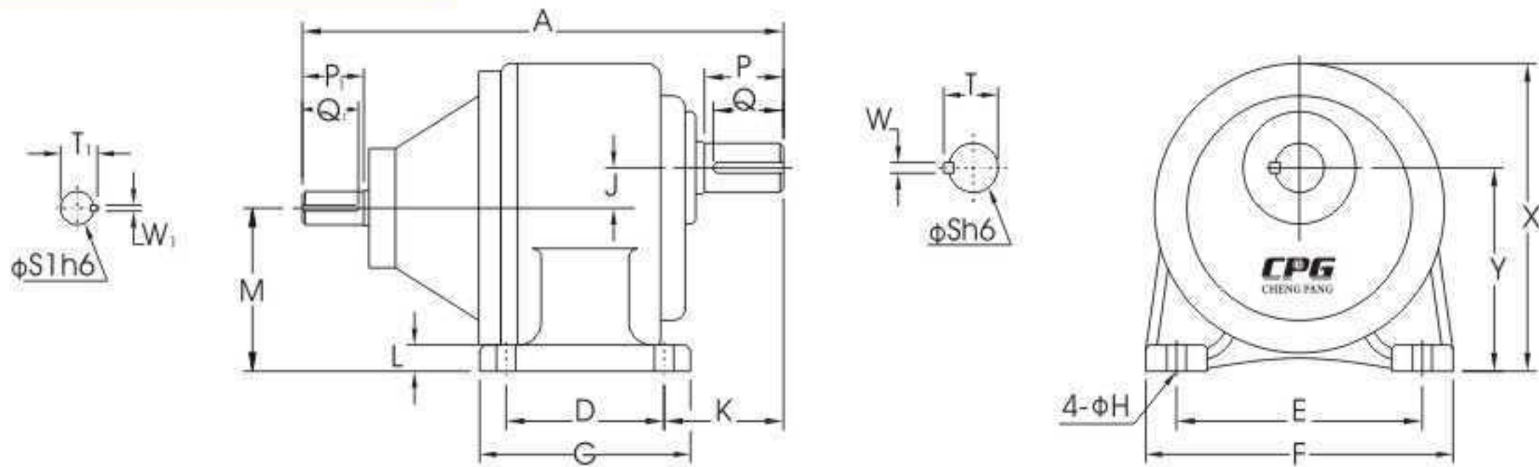
臥式雙軸 HORIZONTAL TYPE
