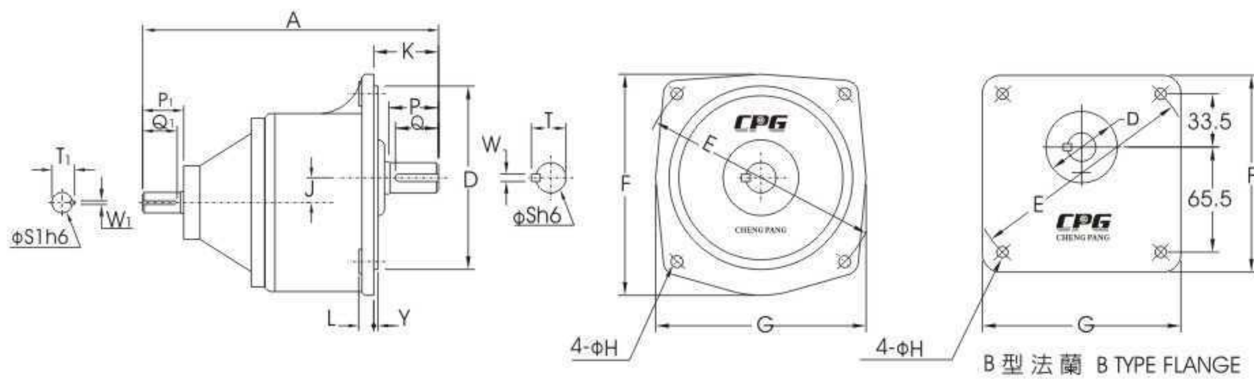
立式雙軸 VERTICAL TYPE
