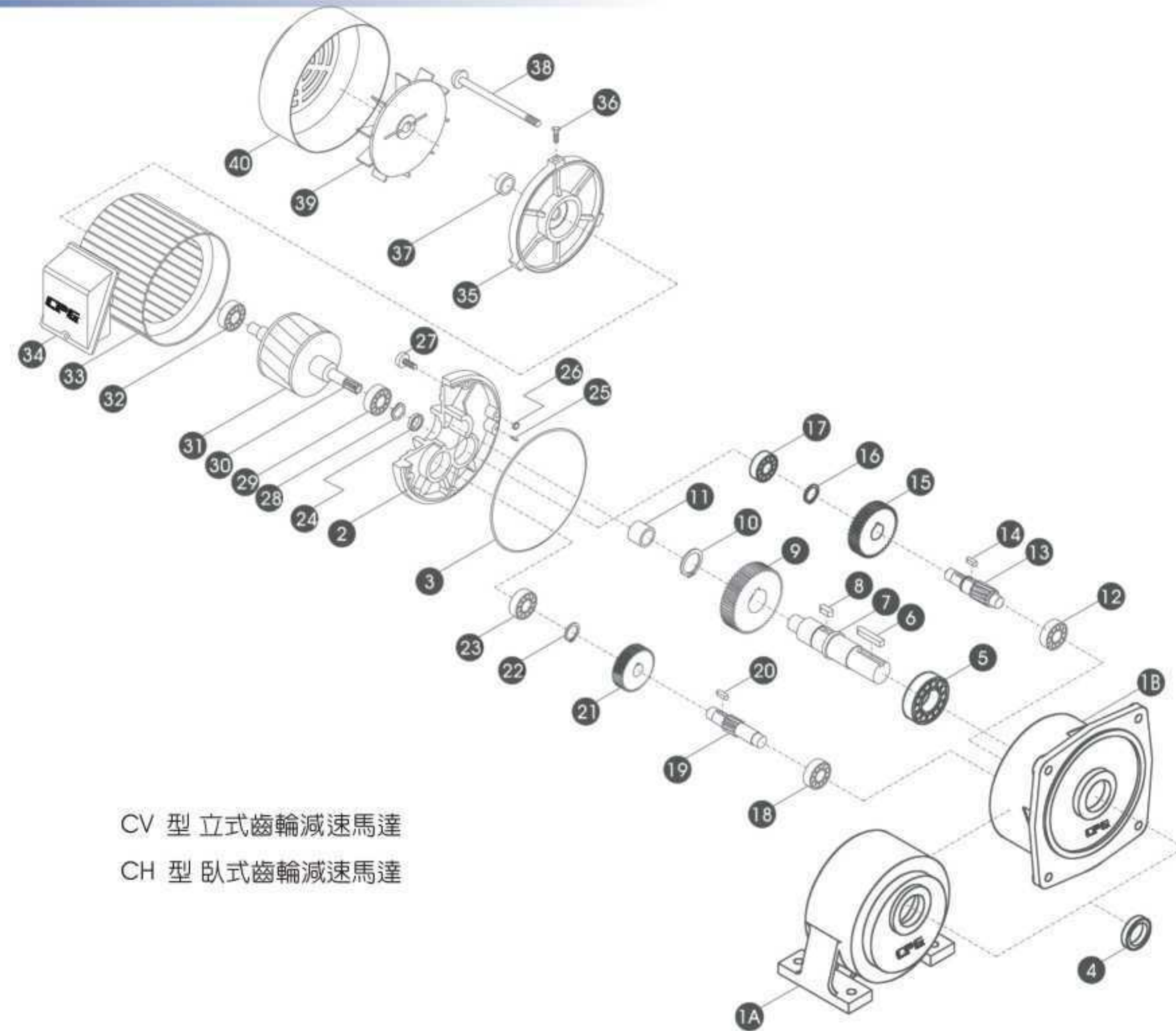
2段/3段式結構剖示圖 2 STAGES / 3 STAGES SECTIONAL DIAGRAM
